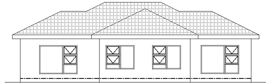
EAST ELEVATION SCALE 1:100
