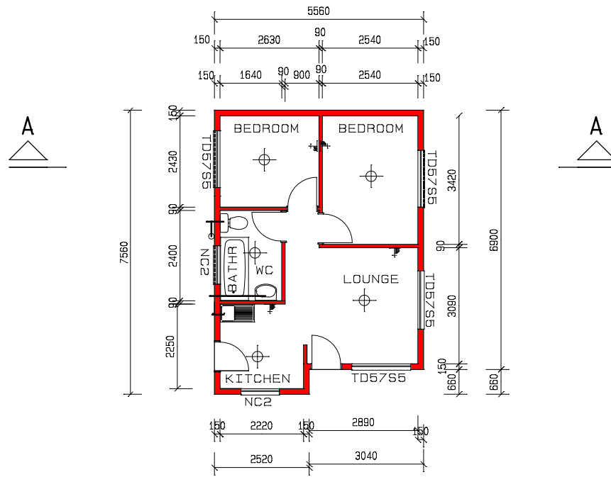
FLOORPLAN 40m 2 SCALE 1:100
