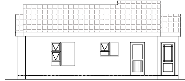
SOUTH ELEVATION
