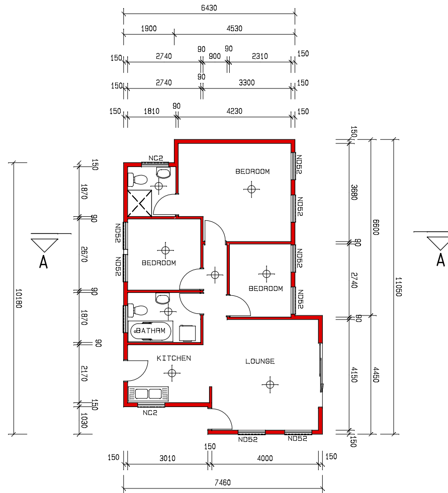
FLOORPLAN 70m 2
