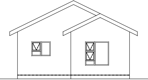
EAST ELEVATION
