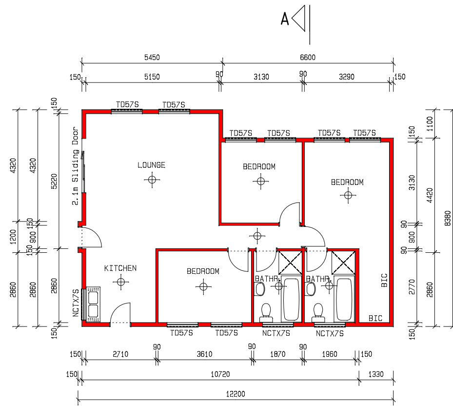
FLOORPLAN SCALE 1:100 90m 2
