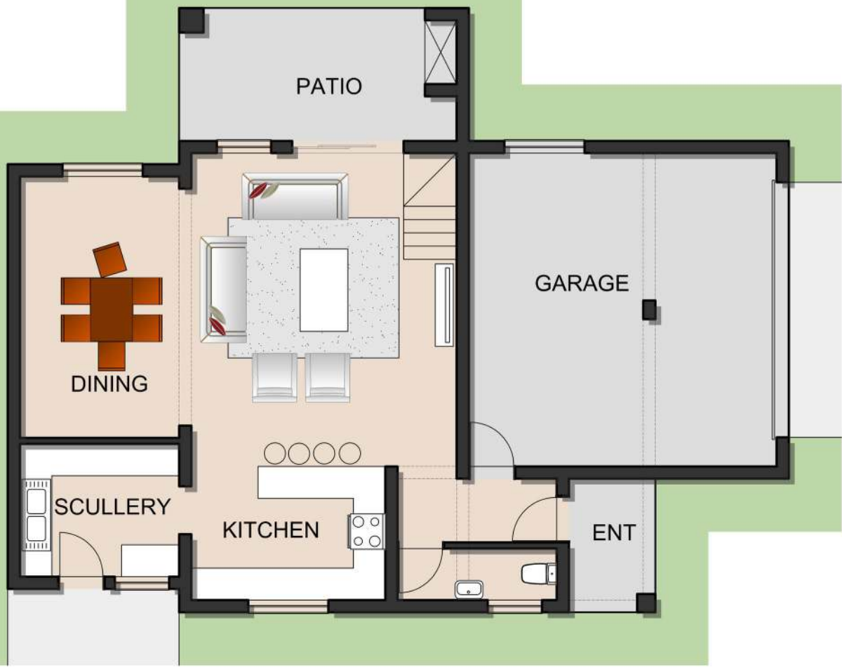
TYPE F GROUND STOREY scale 1:100
